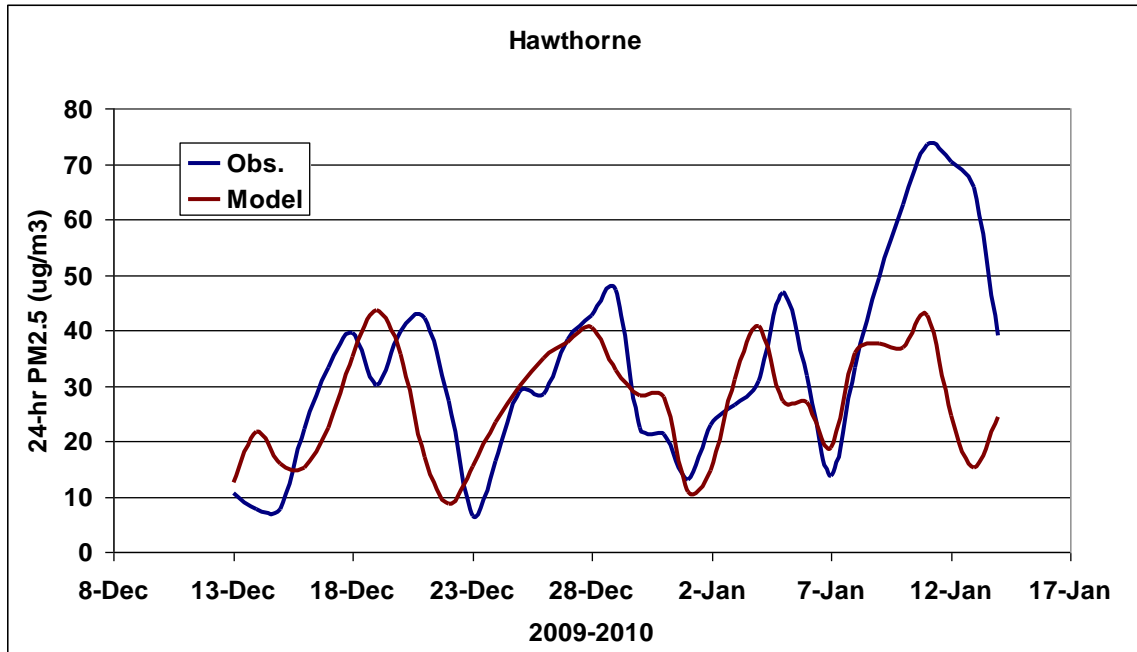
Figure 5.7: 24-hr PM_{2.5} time series (Hawthorne). Observed 24-hr PM_{2.5} (blue trace) and CMAQ modeled 24-hr PM_{2.5} (red trace).
