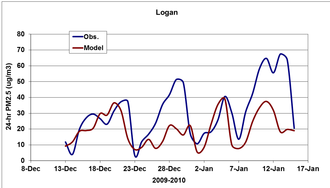
Figure 5.10: 24-hr PM 2.5 time series (Logan). Observed 24-hr PM 2.5 (blue trace) and CMAQ modeled 24-hr PM 2.5 (red trace).
